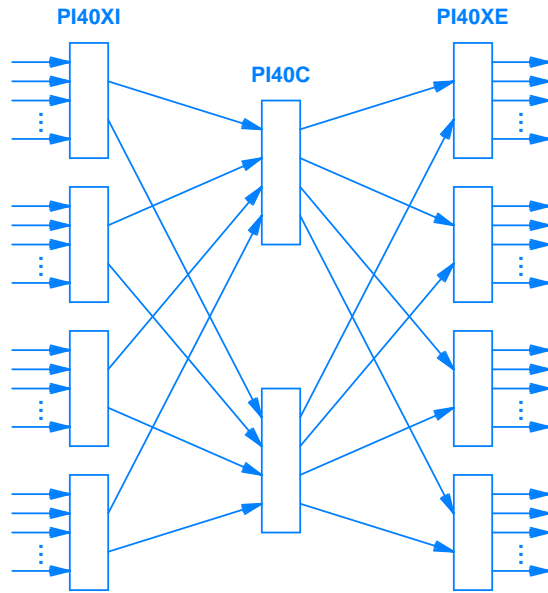
Figure 10.11 Illustration of an Agere switching fabric that uses two PI40Cs and eight PI40Xs either configured for input or output. A PI40XI selects between the two PI40Cs at random.
