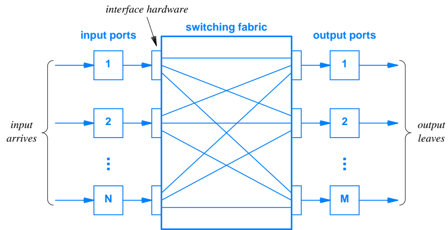
Figure 10.2 Illustration of a fabric that contains a separate physical data path for each interconnection. Interface hardware is needed to allow a port to specify the path for data being sent.
