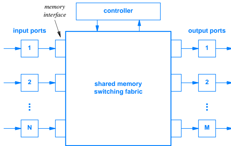
Figure 10.6 Illustration of a switching fabric that uses shared memory. The memory is used to pass data; a separate hardware controller is used to pass coordination and control information.
