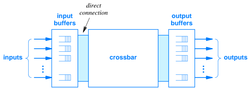
Figure 10.9 The conceptual organization of the Agere switching fabric. Input and output units contain buffers for up to 8K bytes of data.
