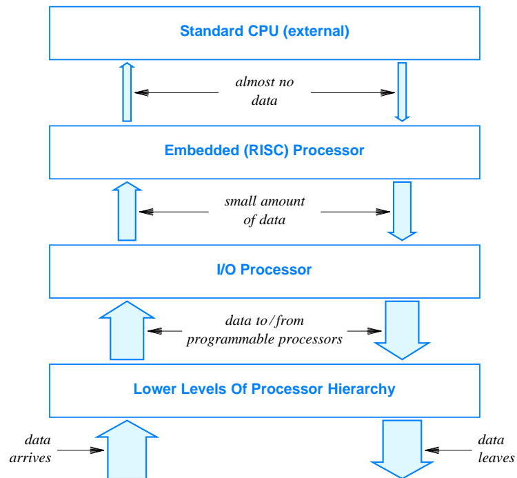
Figure 13.7 Illustration of packet flow through the processor hierarchy. Performance is maximized when lower levels handle packets locally without passing them up the hierarchy.
