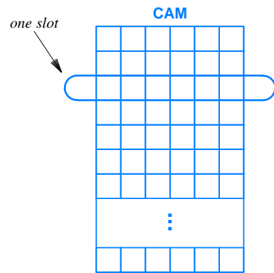
Figure 14.5 Illustration of content addressable memory organized into a two-dimensional array. Each row in the array corresponds to a slot of the memory.
