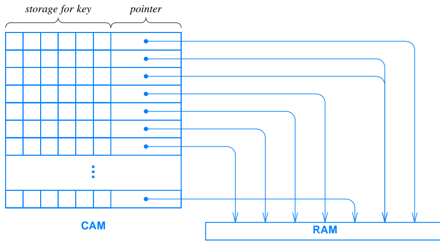
Figure 14.7 Illustration of an associative memory constructed from a CAM. Each slot in the CAM contains a pointer to information in RAM.
