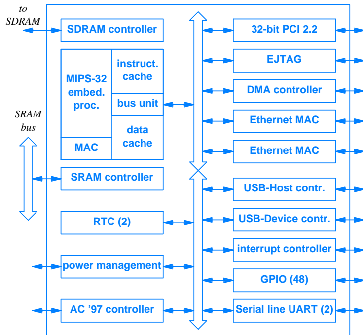
Figure 15.1 The internal architecture of Alchemy's Au1500 chip. Two internal buses provide interconnections: a system bus (the top bus) and a peripheral bus (the bottom bus).
