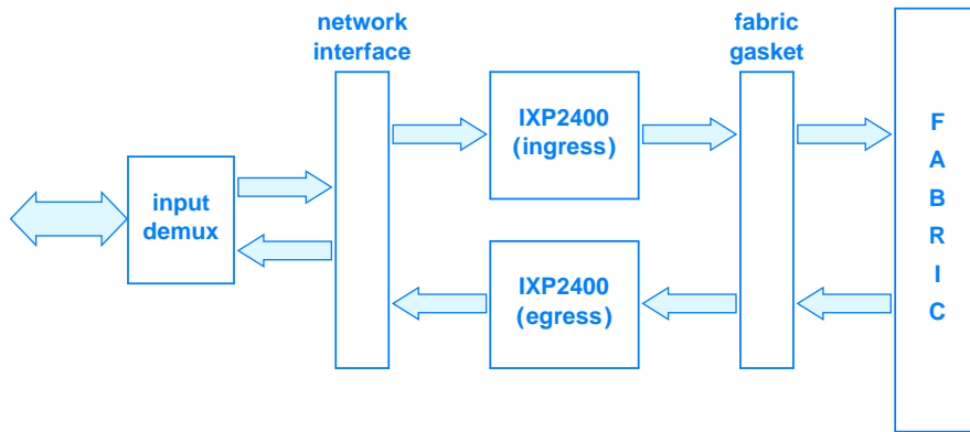
Figure 15.11 Illustration of two IXP2400 chips in a high-speed configuration. One chip handles ingress; the other handles egress.
