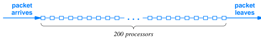
Figure 15.15 The conceptual architecture of an Xelerated network processor. A packet passes through a pipeline of 200 processors.
