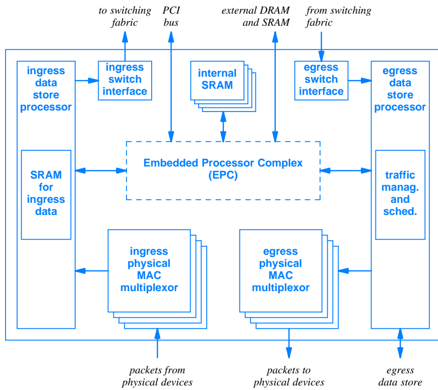
Figure 15.6 The internal architecture of an IBM PowerNP network processor. The high-level diagram hides details such as the structure of the area labeled Embedded Processor Complex and additional external connections.
