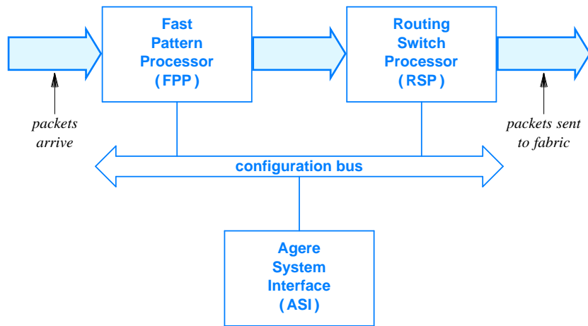
Figure 17.2 First generation implementation of Agere's PayloadPlus network processor architecture. Each functional block is implemented with a separate chip.
