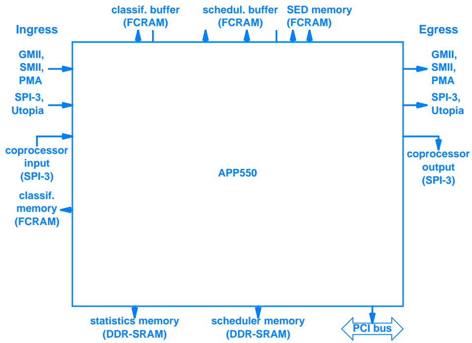
Figure 17.6 Illustration of the major external connections for an Agere APP550 network processor.
