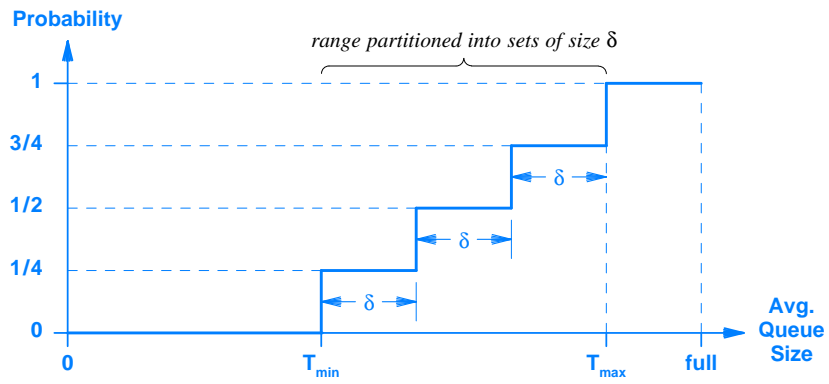
Figure 22.4 A plot of the approximation used to implement Equation 22.2. Using the stair step means that neither floating point computation nor integer division is required.
