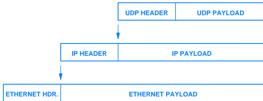
Figure 3.11 Illustration of encapsulation. A UDP datagram travels in an IP datagram, which is encapsulated in an Ethernet frame during transport across one network.
