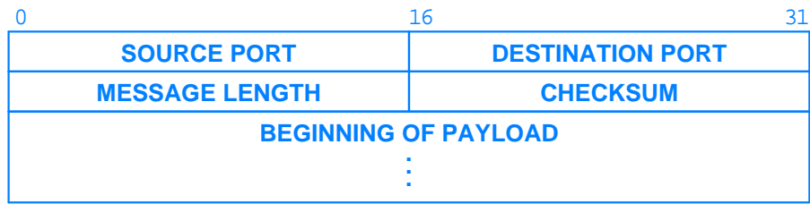
Figure 3.7 UDP user datagram format.
