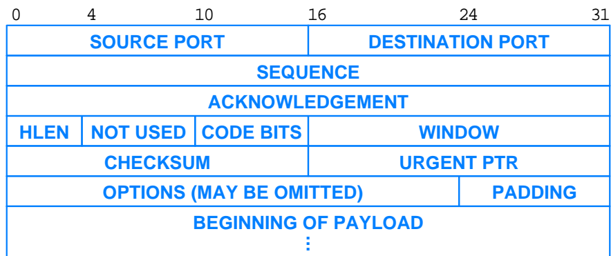
Figure 3.9 The TCP segment format.
