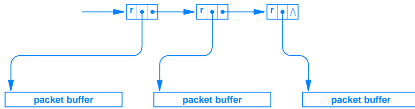
Figure 4.4 An example linked list of commands in memory. Each node on the list specifies an operation ( transmit or receive ), a pointer to a buffer in memory (or a list of buffers if data chaining is used), and a pointer to the next command.
