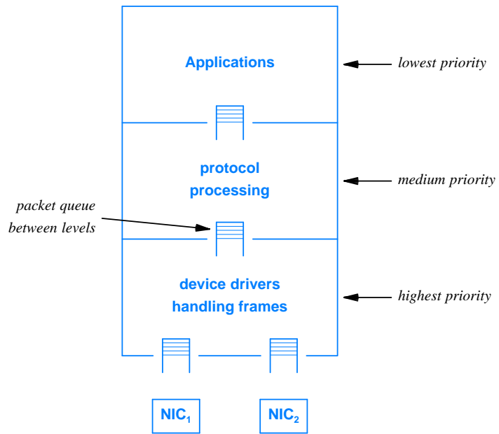
Figure 7.1 Conceptual processing priorities when using a software interrupt mechanism. A packet queue provides the interface between each priority level.
