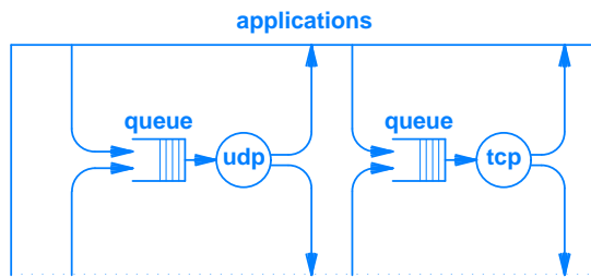
Figure 7.3 An illustration of one thread per protocol at layer 4. Software in adjacent layers must choose one of the two queues when depositing a packet.
