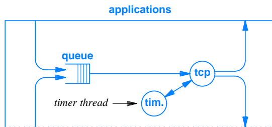
Figure 7.4 Illustration of a separate timer thread used with TCP. The timer manages events such as segment retransmission and maximum segment lifetime timeout, and notifies the TCP thread whenever an event must occur.
