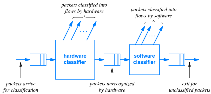
Figure 9.3 Conceptual architecture of a hybrid classification system. In general, the hardware stage handles standard packets and the software stage handles exceptions.
