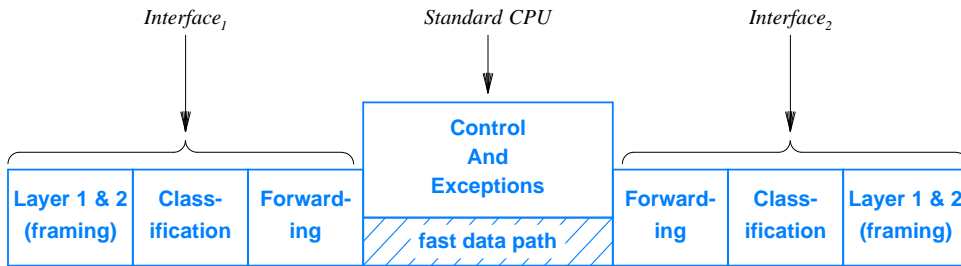
Figure 9.4 The conceptual organization of a second generation network system with more powerful interfaces. An input interface forwards most packets across a fast data path to the appropriate output interface; the central CPU is used to handle exceptions and errors.
