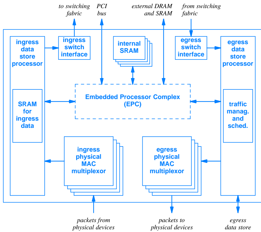
Figure 15.12 The internal architecture of an IBM PowerNP network processor. The high-level diagram hides details such as the structure of the area labeled Embedded Processor Complex and additional external connections.
