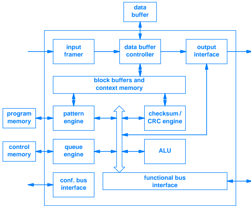
Figure 15.2 The internal architecture of Agere's FPP chip. Packets arrive at the input framer, and leave via the output interface.
