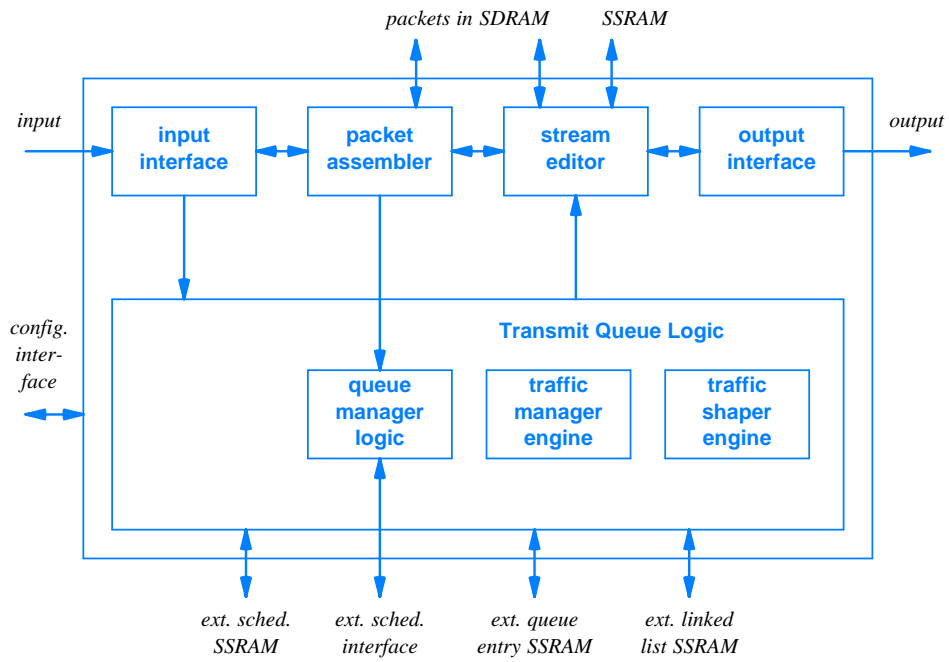
Figure 15.4 The internal architecture of Agere's RSP chip. Packets arrive from the FPP chip after they have been classified.
