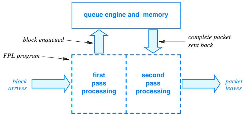
Figure 16.8 Illustration of the conceptual flow of data through an FPL program. The first pass is invoked once for each block; the second pass is invoked once for a packet.
