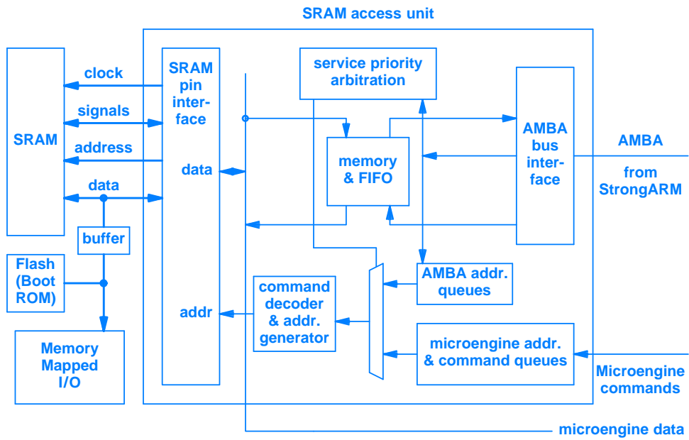
Figure 18.10 Some of the detail in the SRAM access unit found on Intel's IXP1200 network processor.
