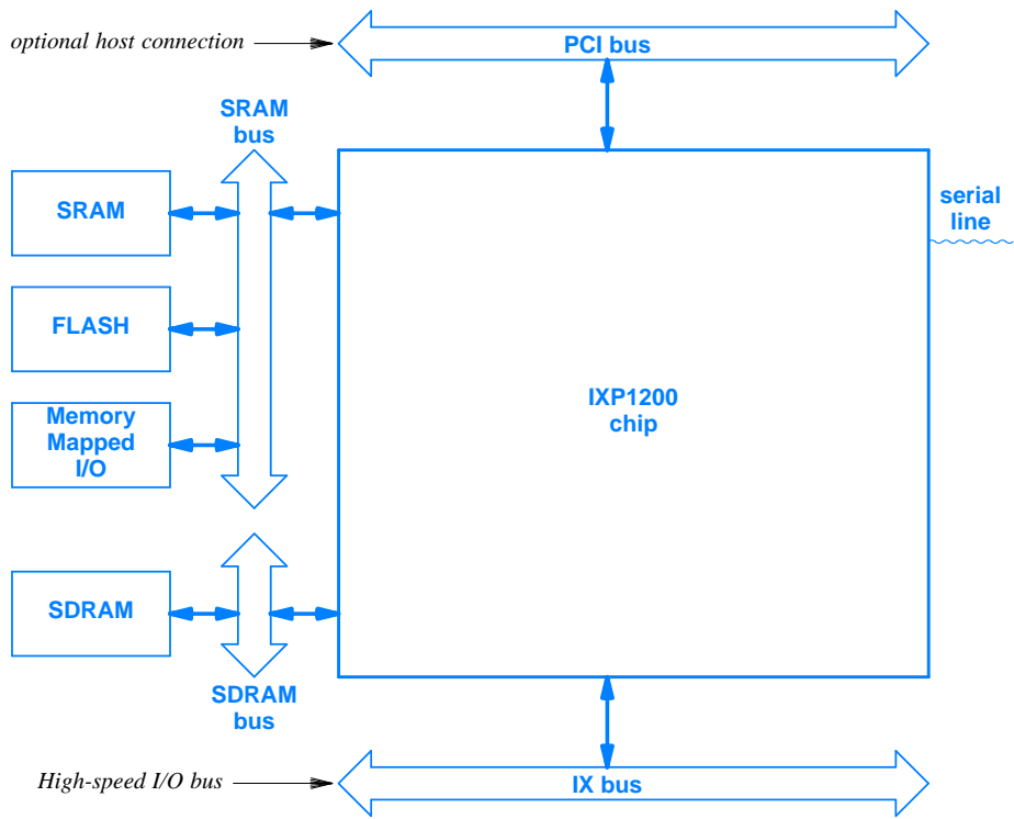
Figure 18.3 Illustration of the external connections for an Intel IXP1200 network processor.
