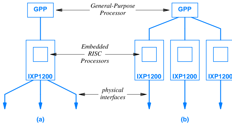
Figure 19.1 Illustration of two possible systems designs: (a) a single IXP1200 that handles multiple network interfaces, and (b) multiple IXP1200s each dedicated to a single network interface. The tasks assigned to the embedded RISC processor depend on the design.
