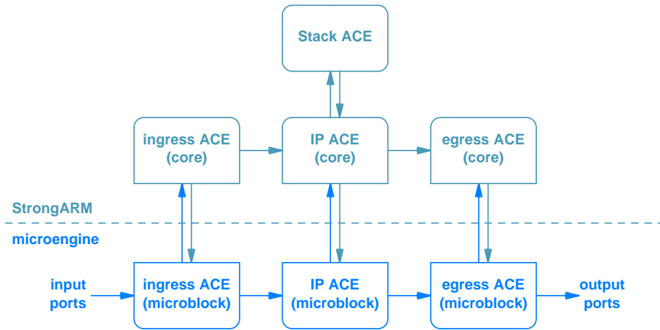
Figure 22.2 Illustration of a system in which three ACEs contain both a core component and a microblock component. The Stack ACE does not contain a microblock component.
