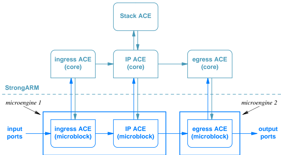
Figure 22.3 Illustration of microblocks collected together into microblock groups. Each group corresponds to the code that executes on a microengine.
