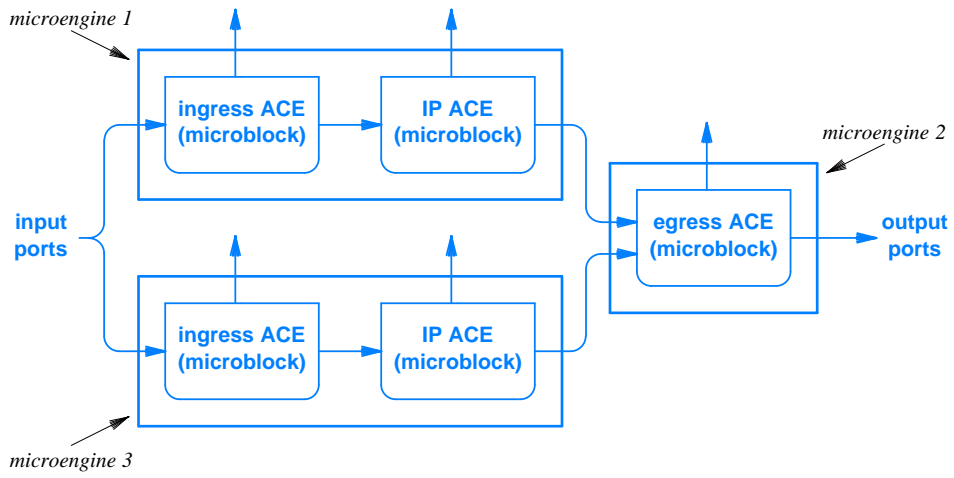
Figure 22.4 Illustration of a microblock group replicated on microengines 1 and 3. Both copies of a microACE connect to the same core component, and both copies share access to input devices.
