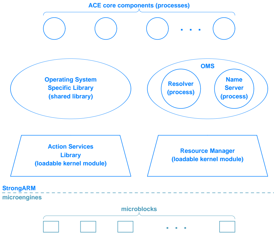
Figure 23.2 Principle components in Intel's run-time system that support ACE execution, and the implementation used for each.
