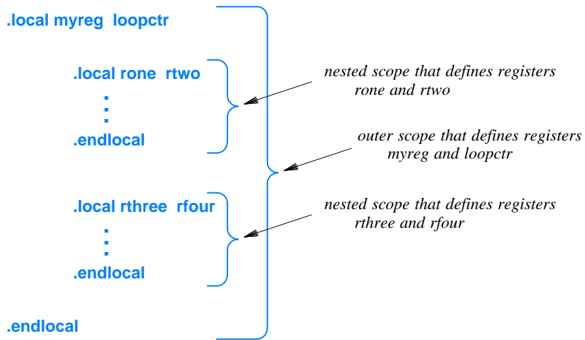
Figure 24.5 An example of nested scope declarations and the set of register names that are known in each. Although it is not required, indentation helps a programmer understand the nesting.
