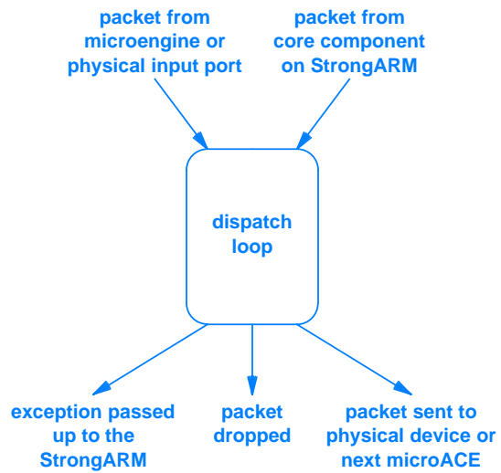
Figure 25.3 Illustration of the packet sources and sinks in a typical dispatch loop used with the Intel SDK. The dispatch loop repeatedly checks each source, processes a packet, and then chooses one of the sinks for the packet.
