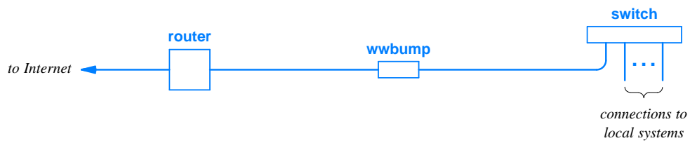
Figure 26.1 An example of a wwbump system inserted into the connection between a router and an Ethernet switch. The wwbump system passes traffic transparently.
