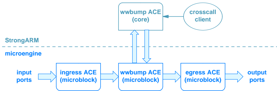
Figure 26.2 Internal structure of ACEs in the wwbump system and the packet flow among them. Web packets are sent to the StrongARM, and other packets flow directly through to the egress ACE.
