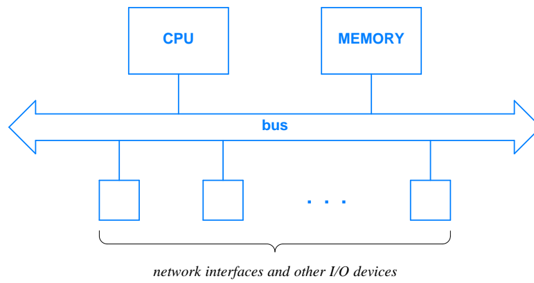
Figure 4.1 Illustration of conventional computer architecture when used for a network system. Network interface hardware attaches to the computer's bus.
