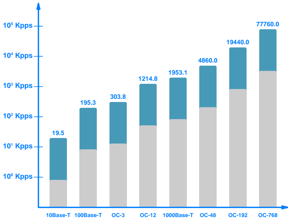
Figure 8.3 Illustration of packet rates on log scale for technologies listed in Figure 8.2. The gray portions show the rates for large packets.
