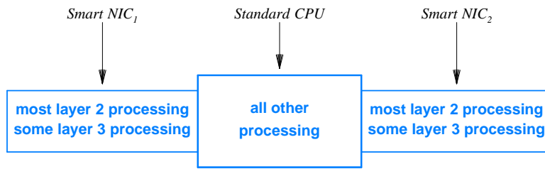
Figure 8.5 Hardware architecture of an optimized system with smart network interface cards. Because each NIC performs more processing, the CPU load is reduced.
