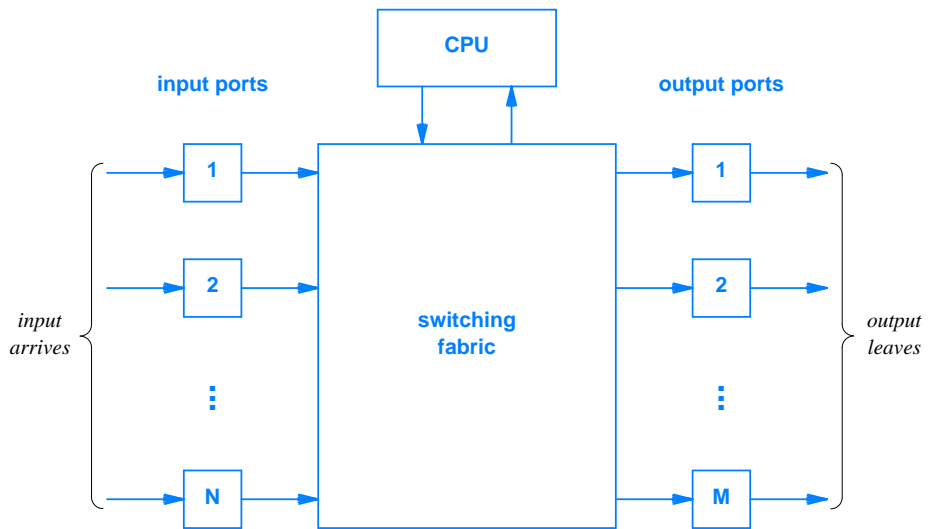
Figure 10.1 The switching fabric concept. The fabric is an internal hardware interconnection mechanism that allows any input port to send to any output port.
