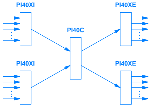
Figure 10.10 An implementation of the Agere switching fabric using multiple chips. The PI40XI and PI40XE consist of the same chip configured for ingress or egress.
