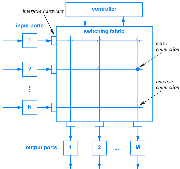
Figure 10.3 Illustration of a crossbar switching fabric shown with an active switch connecting input port 2 and output port M . The controller determines whether a switch is active or inactive.
