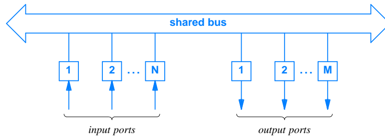
Figure 10.5 Illustration of a shared bus architecture. Each port attaches to the bus over which all transfers occur.
