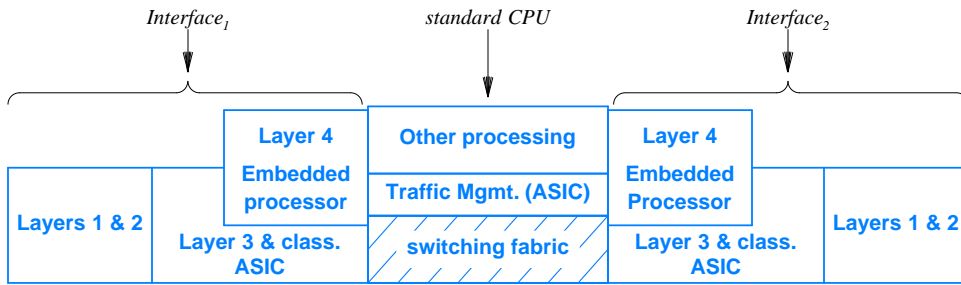
Figure 11.1 Conceptual organization of a third generation network system with an embedded processor plus ASIC† hardware on each interface card. A switching fabric provides the fast data path between interfaces. An interface can handle most of layers 1 through 4, leaving the central CPU free to run applications.
