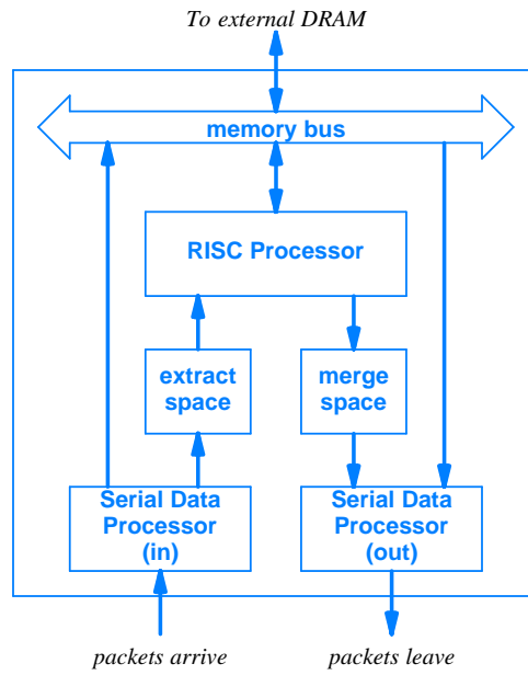
Figure 15.14 The internal architecture of a single CP with a RISC core plus functional units to handle ingress and egress. Each C-Port chip contains a total of sixteen CPs.
