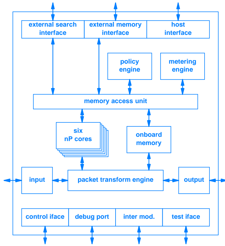
Figure 15.2 The internal architecture of AMCC's nP7510 chip. The chip contains additional interconnections among functional units that are not shown.
