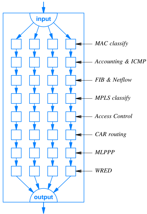
Figure 15.3 An illustration of how Cisco's PXF network processor can be used. Thirty-two embedded processors are partitioned into four separate pipelines.
