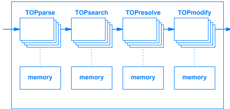
Figure 15.4 Internal architecture of an EZchip NP-1c network processor. Each of the four banks of processors is optimized to perform a specific task.
